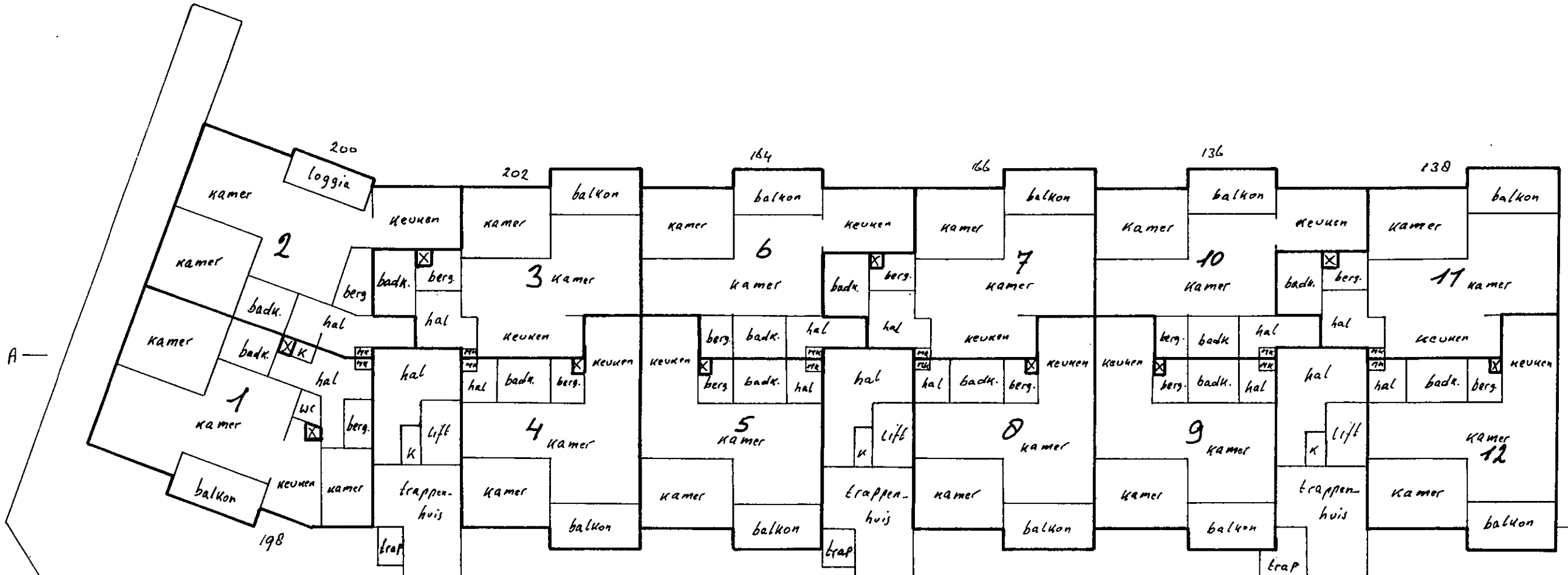
BEGANE GROND 1:200
