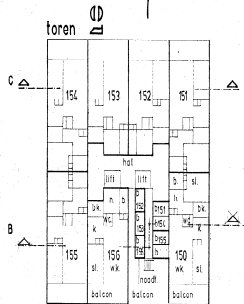
7a Verdieping 1: 200
