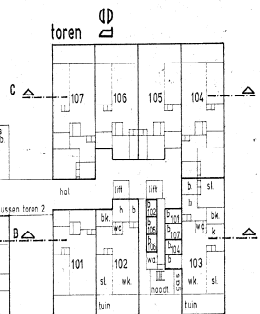
Begane grond 1: 200
