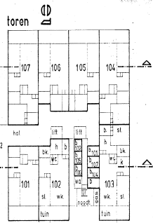
Begane grond 1: 200
