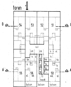
7a Verdieping 1: 200
