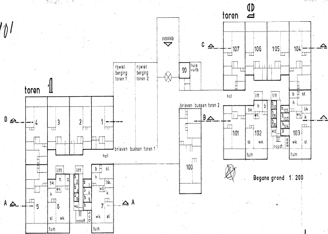
Begane grond 1: 200
