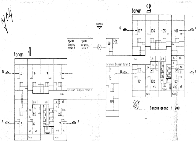
Begane grond 1: 200
