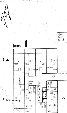
Begane grond 1: 200
