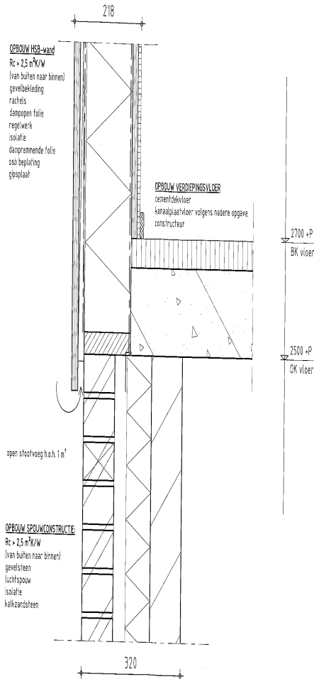
Detail 2
