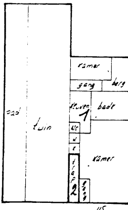
BEGANE GROND 1:200
